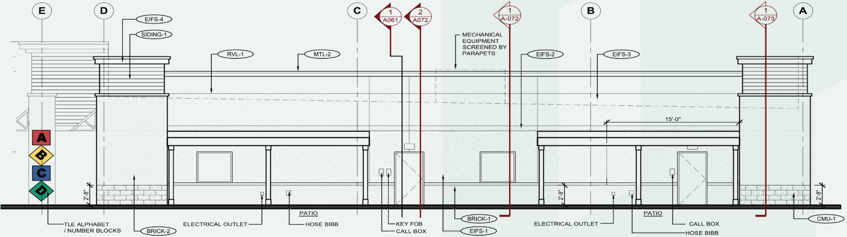
EAST ELEVATION
