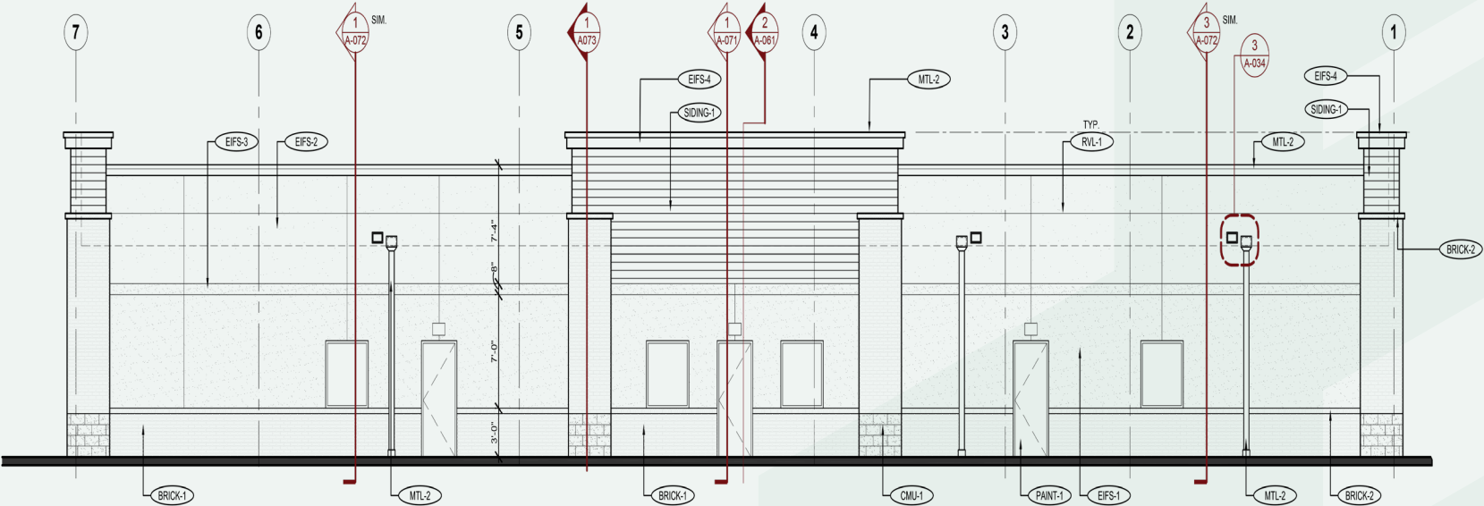
NORTH ELEVATION
